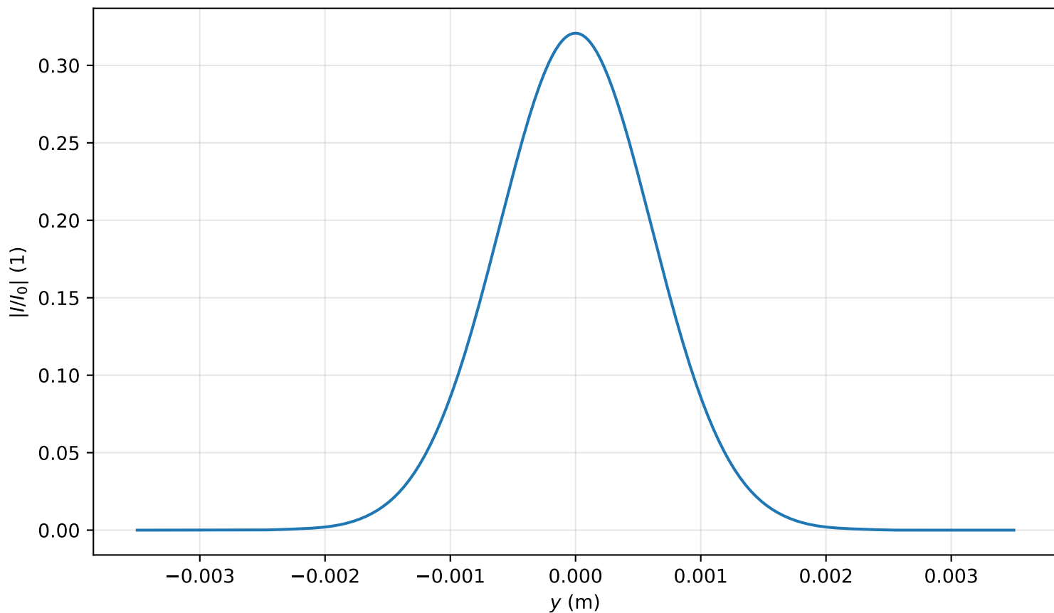
Intensity profile I(x=0, y, z=3.105)/I_0 , P_{in}=0.1P_{cr} , artificial time
